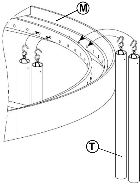
Drawing 2 - Tube Assembly
