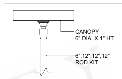
CANOPY DETAIL
