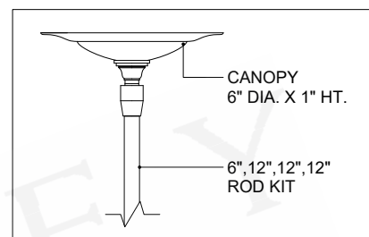
CANOPY DETAIL
