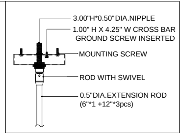
CANOPY DETAIL
