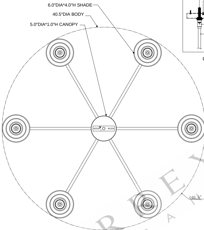
TOP VIEW
